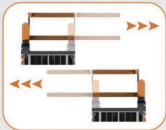
As long as the aisle width is sufficient, it can work both inside and outside the aisle at the same time. One button back to the center (fork position back to the center and facing forward direction) and one button linkage (realize picking up and side shifting function at the same time) are equipped as standard.
